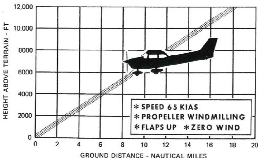
Figure 3-1. Maximum Glide
