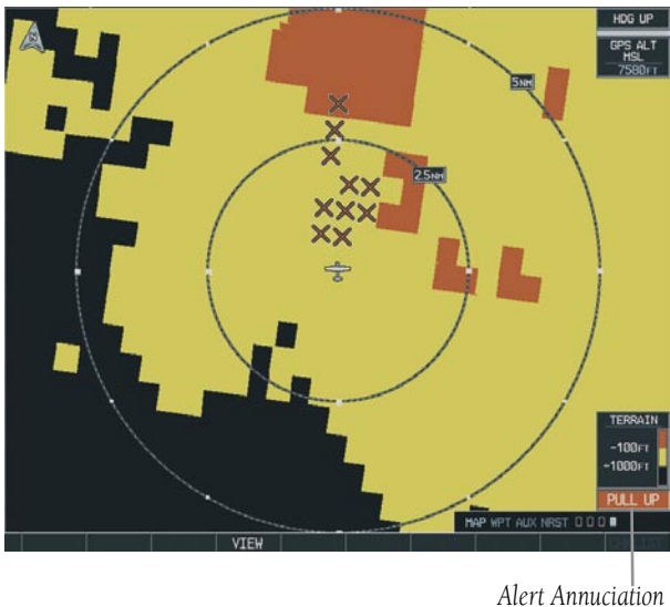
Figure 10-27 Alert Annunciation on the TAWS Page
