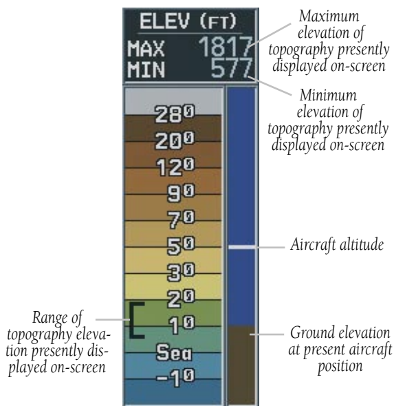
Figure 10-24 Topography Scale
